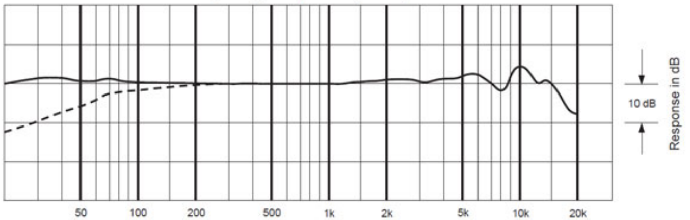
Frequency Response (Omni)
