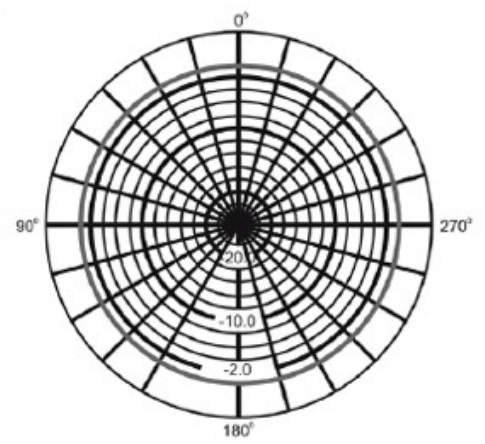
Omnidirectional at 1kHz
